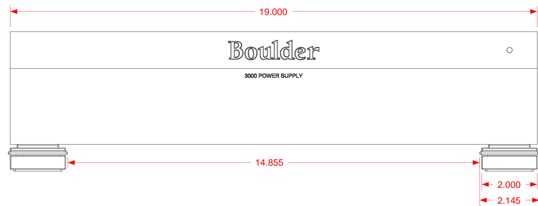
FRONT VIEW SCALE 1:2
