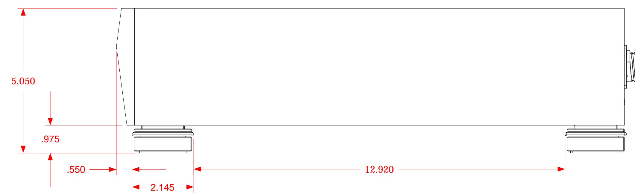
RIGHT SIDE SCALE 1:2
