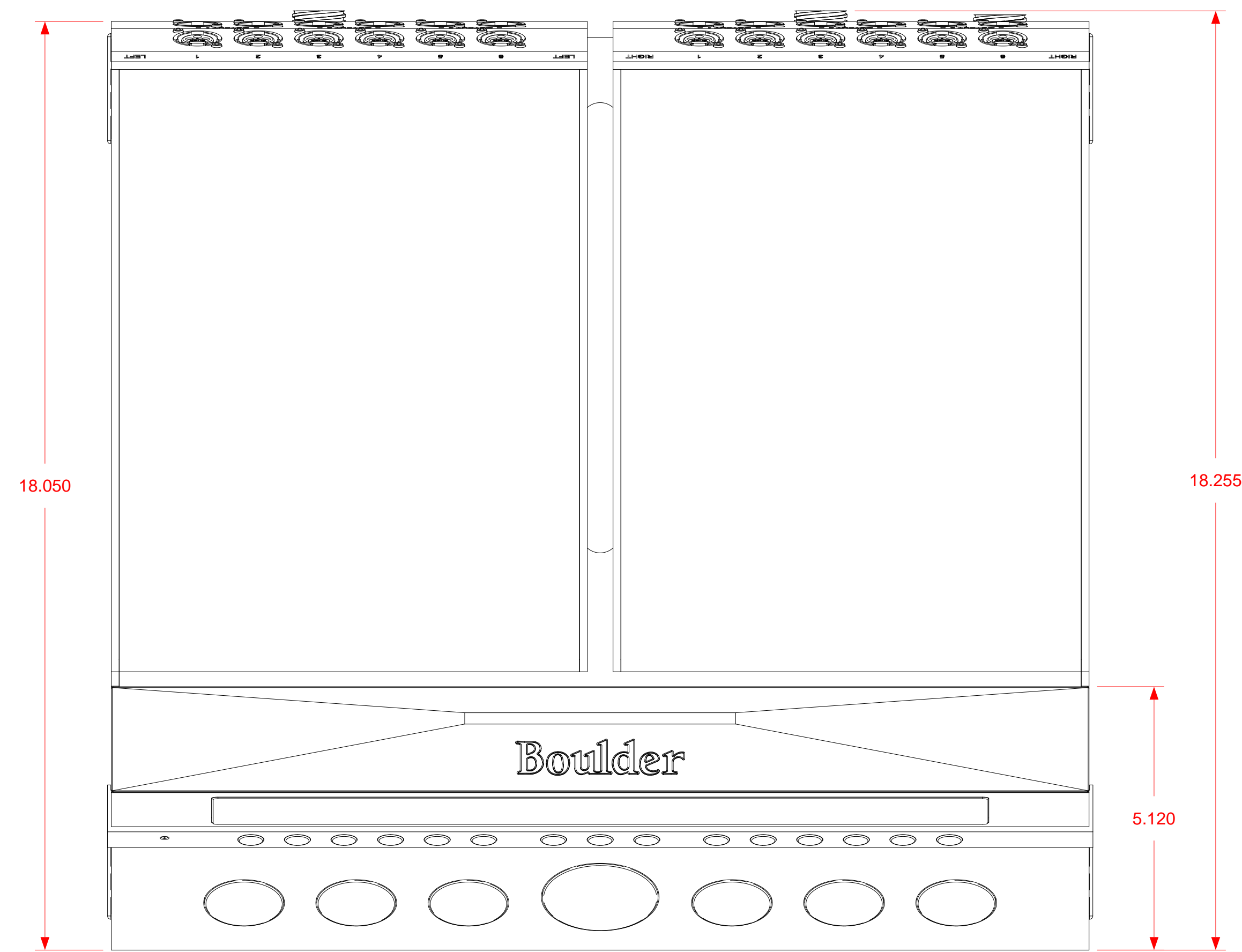
TOP VIEW SCALE 1 : 2
