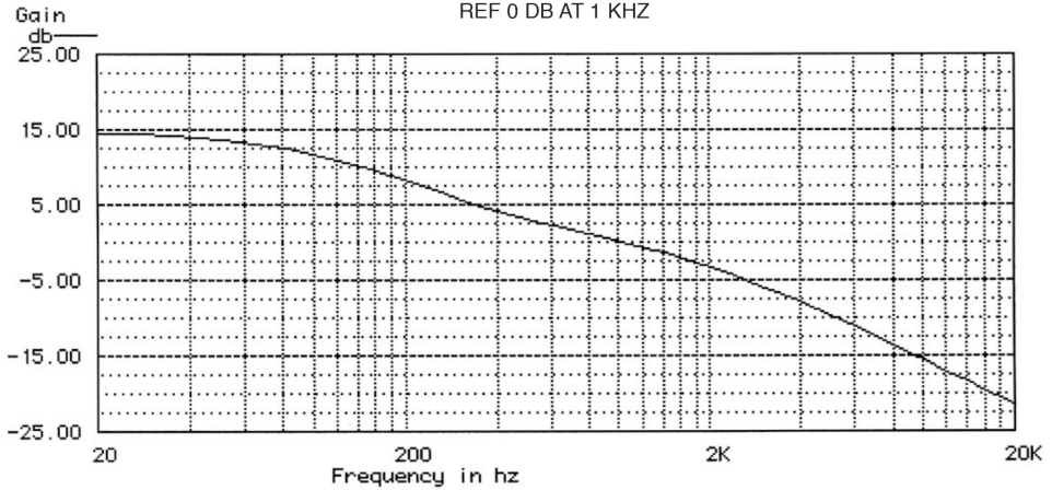
COLUMBIA REPRODUCE EQUALIZATION REF 0 DB AT 1 KHZ
