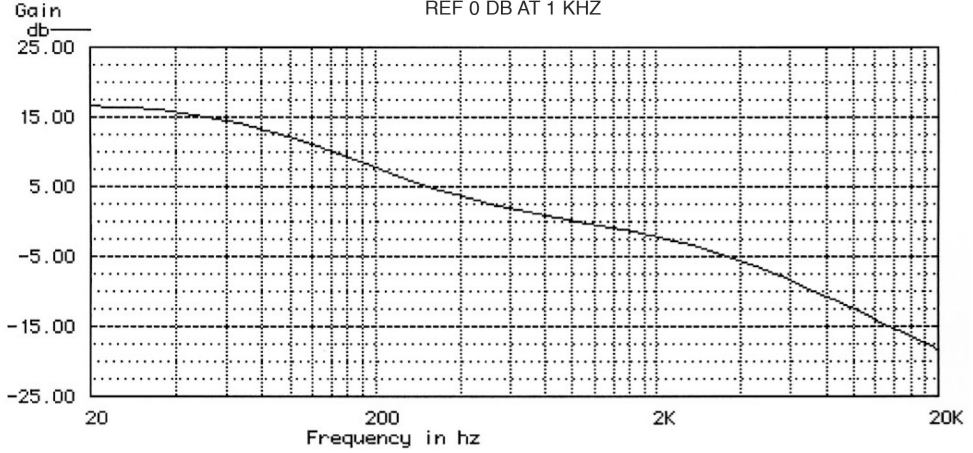
EMI REPRODUCE EQUALIZATION REF 0 DB AT 1 KHZ
